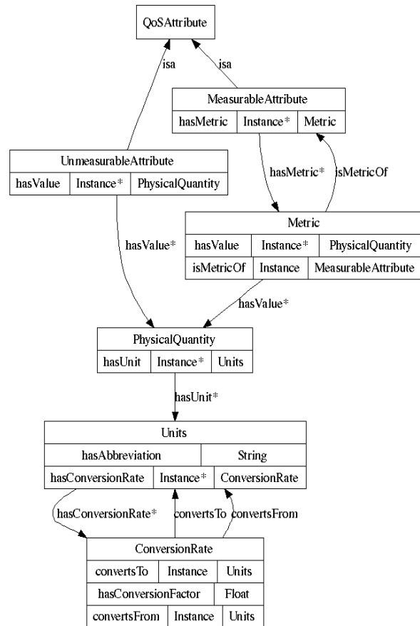
Figure 2. The Base QoS ontology
