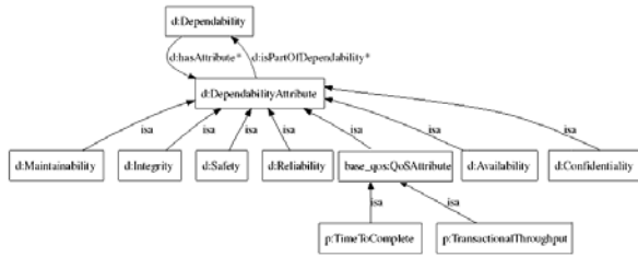
Figure 3. Example Classes from the attribute layer
