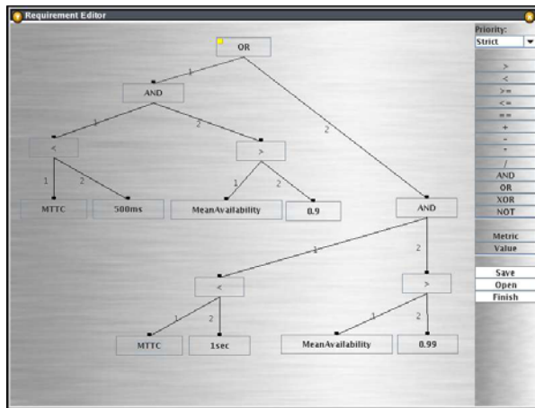
Figure 6. Requirement construction
