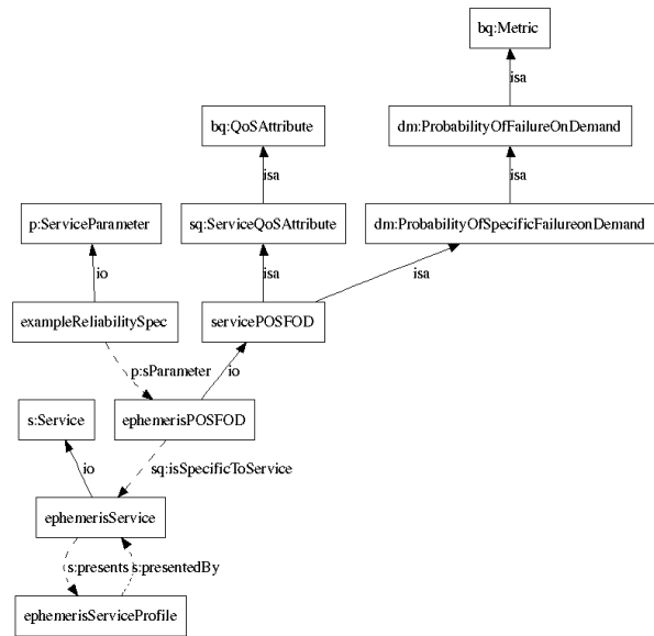
Figure 4. Example of the QoSOnt/OWL-S link
