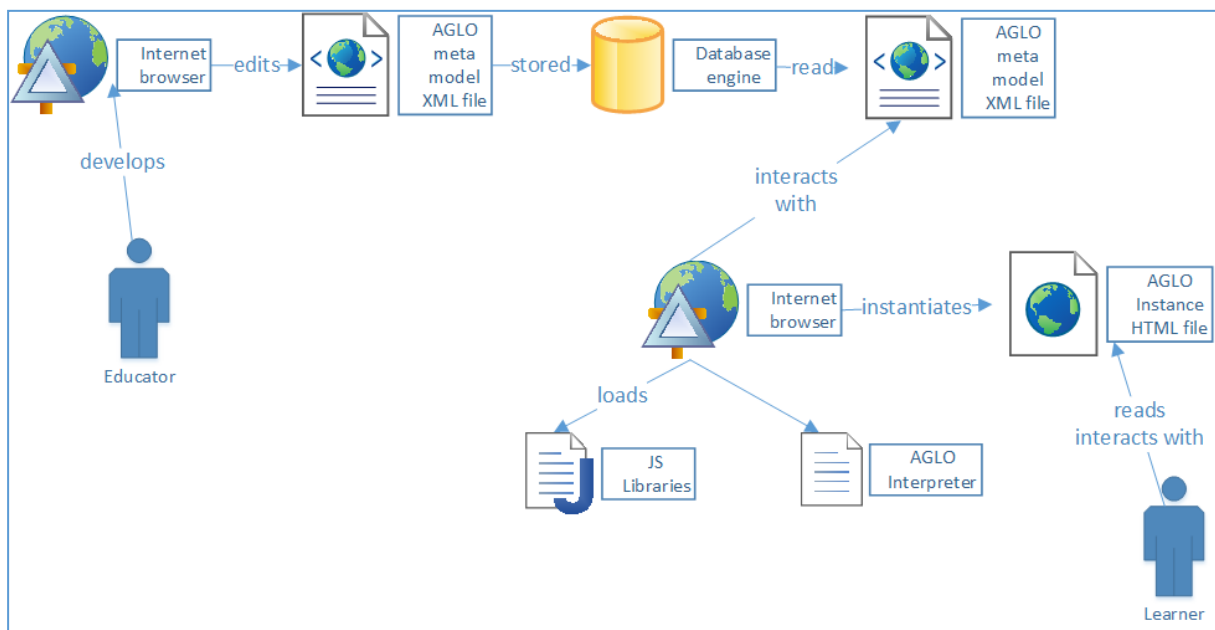
Figure 1 – The GLO Workflow
