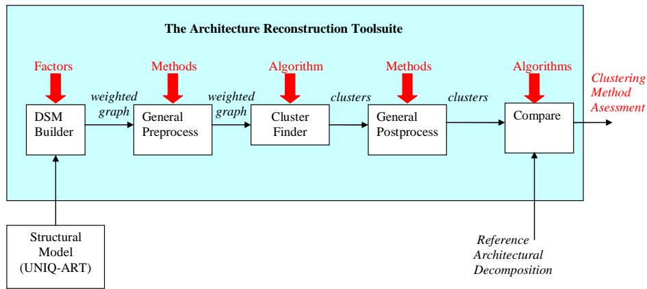
Fig. 1. The Architectural Reconstruction Toolsuite (ARTs)
