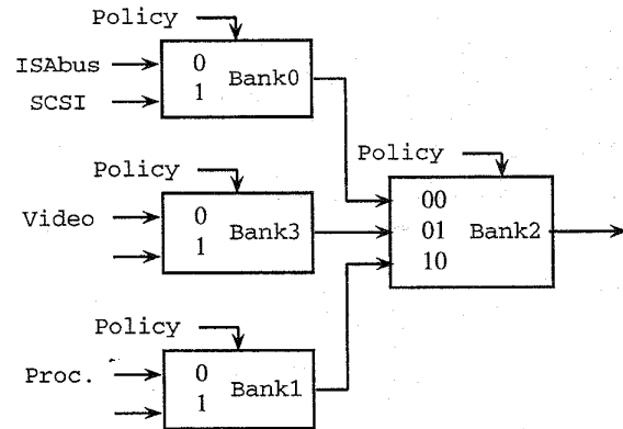
Figure 6: The PCI arbiter
