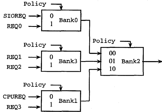
Figure 4: The PCI arbiter
