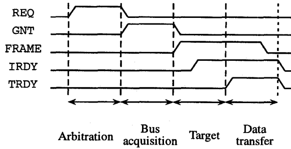
Figure 3: A transaction in the PCI Bus
