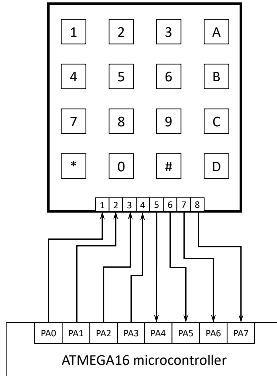
Fig. 4-34 4x4 Microcontroller and keyboard interconnection schematic
