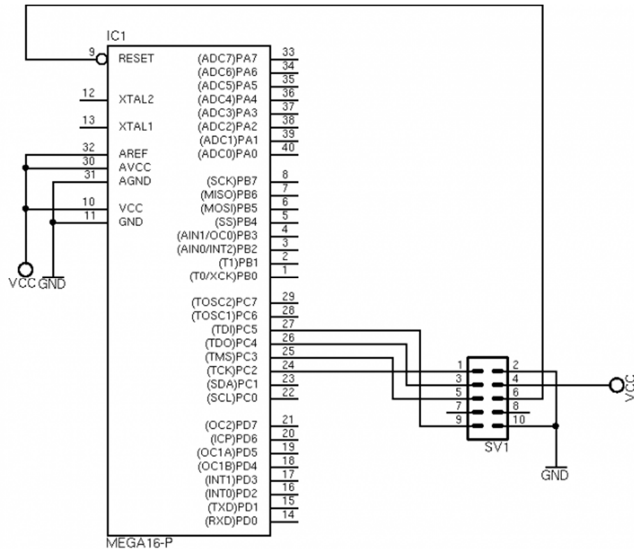
Fig. 4-3 ATMEGA16 JTAG connection
