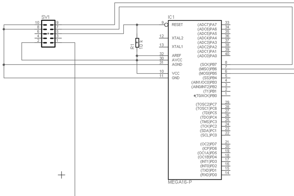
Fig. 2-2 ATMEGA16 ISP connection
