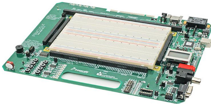
Fig. 4-6 PBMCUSLK peripheral board [16]
