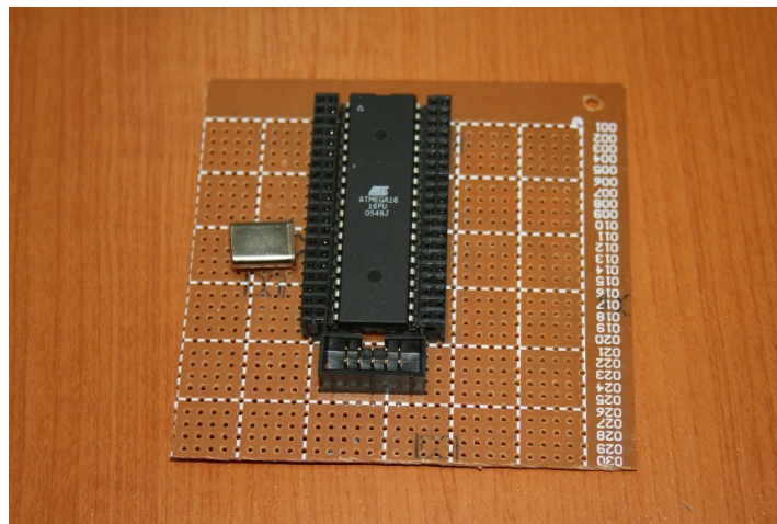
Fig. 2-4 ATMEGA16 header board
