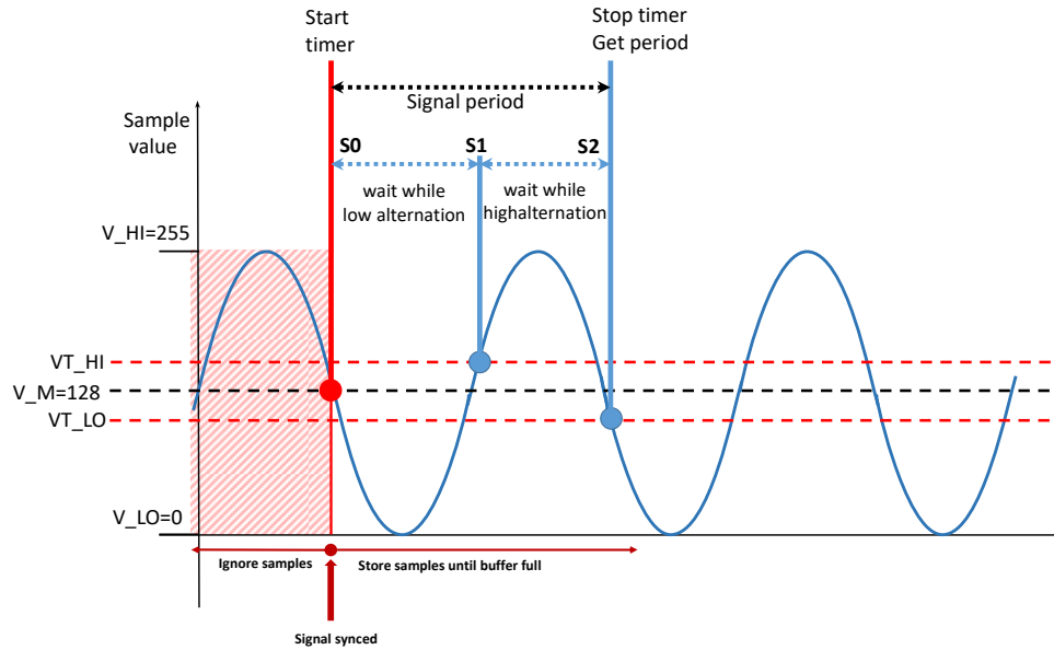
Fig. 2-45 Frequency measurement on negative edge triggering
