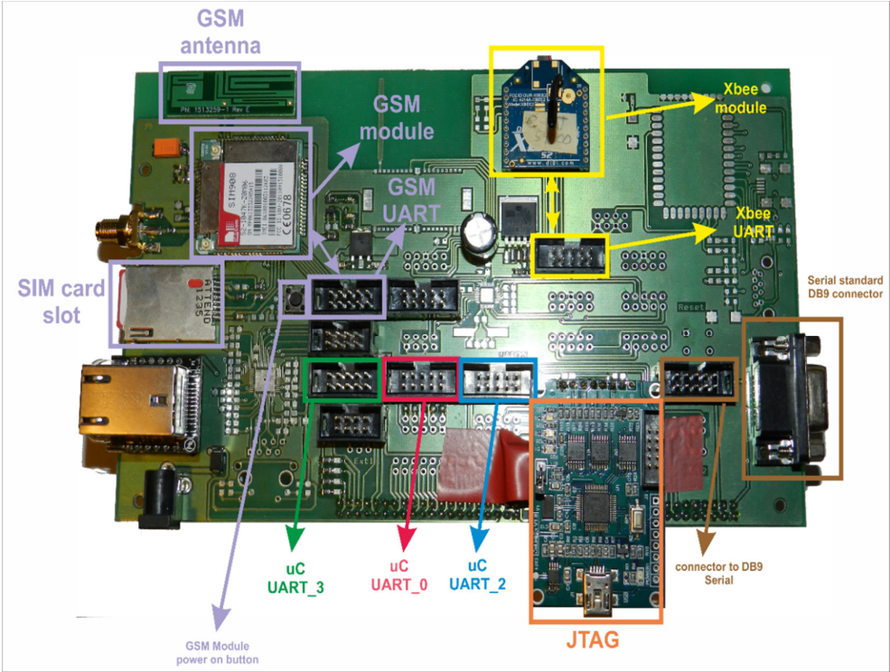
Fig. 1-4 DSPLABS_DT_STK_V1_COMM board component
