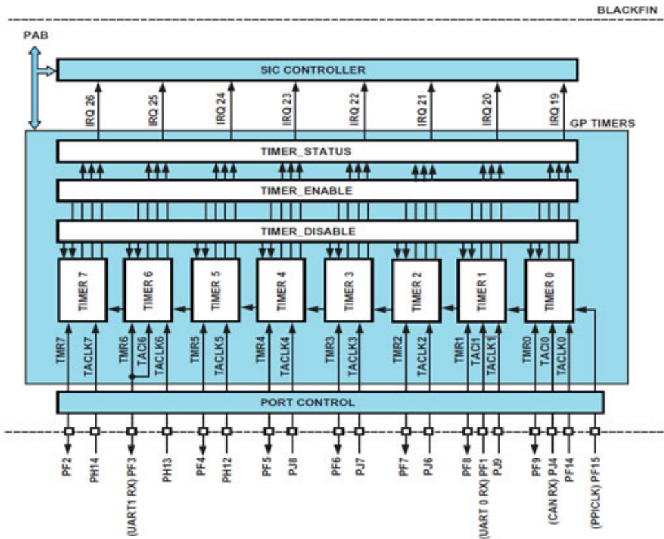
Fig. 3-5 Blackfin BF537 timer block diagram [20]
