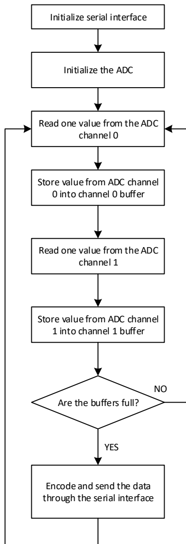
Fig. 2-33 Simple 2 channel oscilloscope program flowchart
