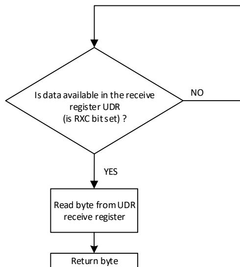
Fig. 2-47 UART receive flowchart
