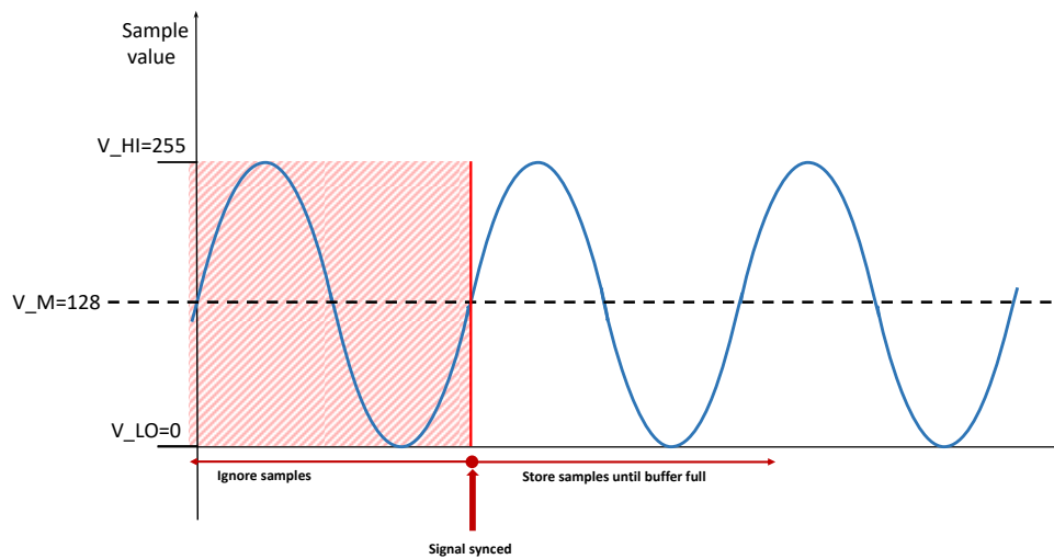
Fig. 2-38 Positive edge trigger using middle value
