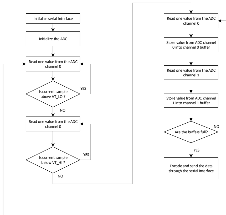
Fig. 2-43 A 2 channel oscilloscope program flowchart with positive edge trigger using instability interval
