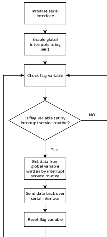
Fig. 4-48 UART echo main program loop with interrupts
