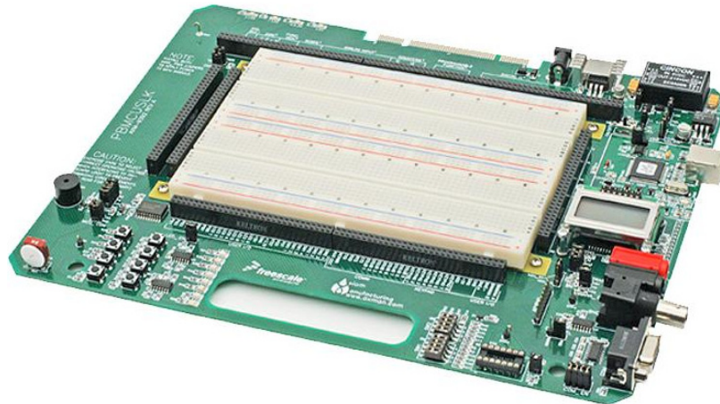
Fig. 2-6 PBMCUSLK peripheral board [16]
