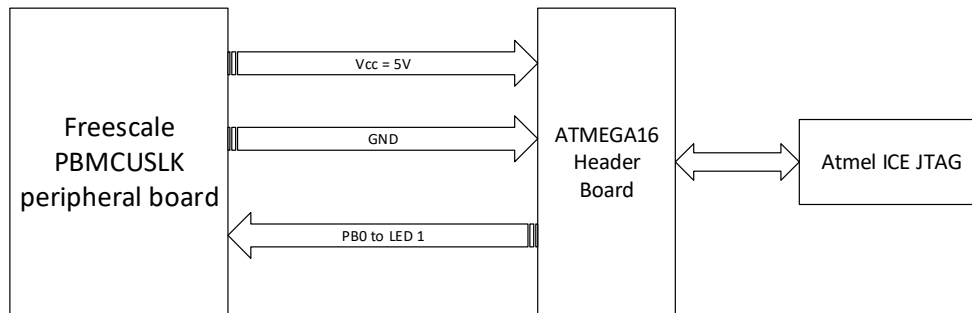
Fig. 4-8 LED blink connection block schematic
