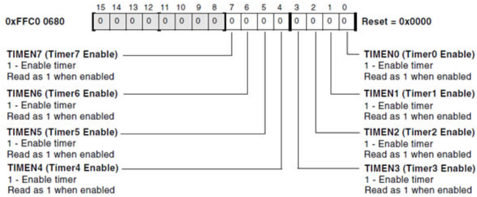
Fig. 3-7 Blackfin BF537 timer enable register structure [20]
