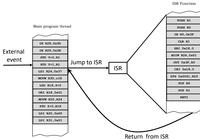
Fig. 4-24 Interrupt diagram
