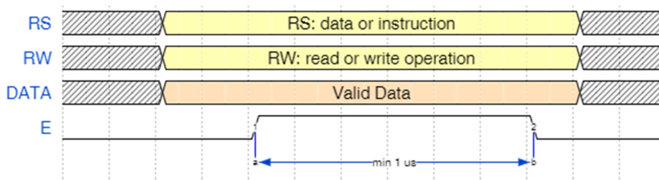
Fig. 4-49 LCD general bus communication example
