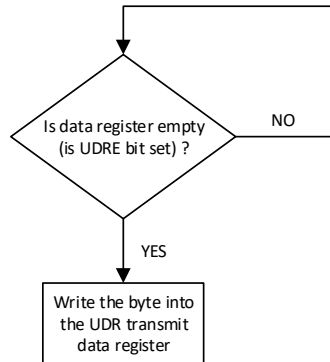
Fig. 2-24 UART transmit flowchart
