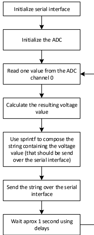
Fig. 4-55 Digital voltmeter program flow
