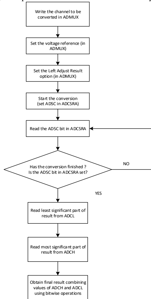
Fig. 4-54 ADC conversion logic
