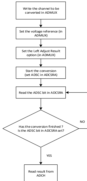
Fig. 2-31 ADC conversion logic
