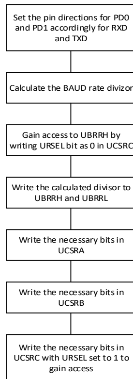
Fig. 2-23 UART initialization flowchart
