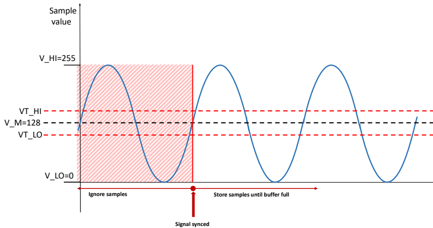
Fig. 2-41 Positive edge trigger using instability interval
