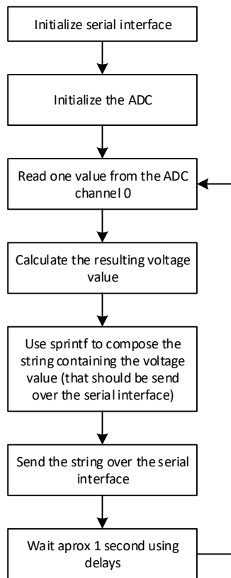
Fig. 2-32 Digital voltmeter program flow
