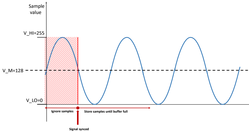
Fig. 2-37 Negative edge trigger using middle value
