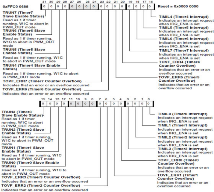
Fig. 3-8 Blackfin BF537 timer status register structure [20]
