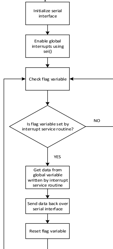
Fig. 2-49 UART echo main program loop with interrupts
