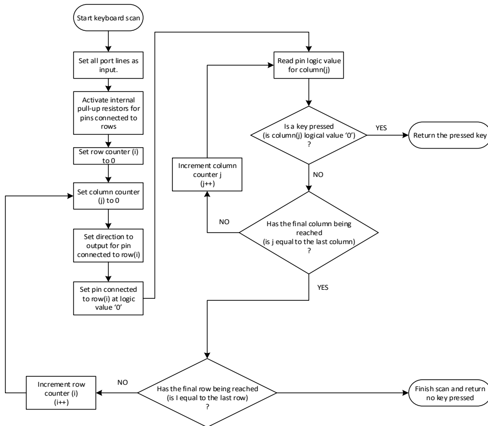
Fig. 4-35 Matrix keyboard scan algorithm
