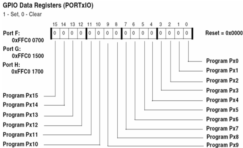
Fig. 3-2 GPIO Input / Output registers description [20]
