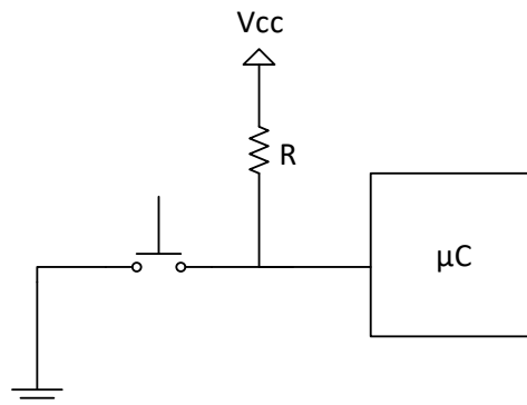
Fig. 4-19 Push-button connection to microcontroller GPIO port
