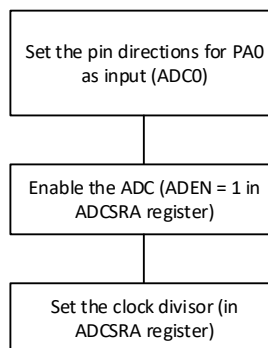
Fig. 4-53 ADC initialization flowchart
