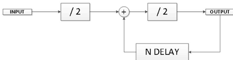
Fig. 3-11 Echo generation system block diagram
