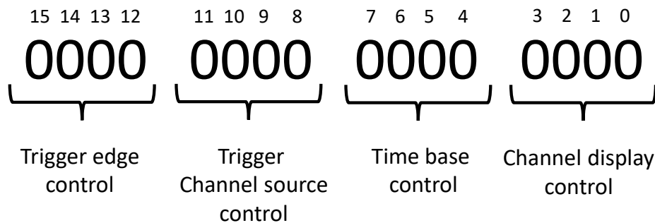
Fig. 2-50 Bitwise command encoding protocol
