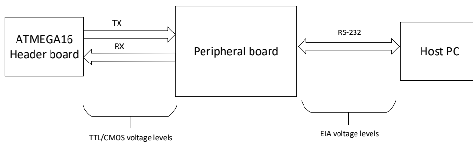
Fig. 2-22 UART connections block diagram
