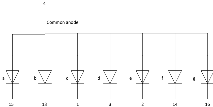
Fig. 4-29 Detailed digit schematic
