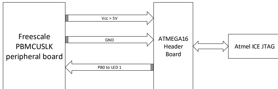
Fig. 2-8 Led blink connection block schematic
