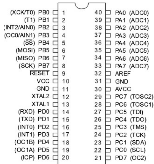
Fig. 2-1 Pinout of ATMEGA16
