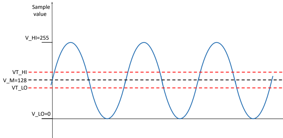
Fig. 2-39 Simple waveform with instability interval
