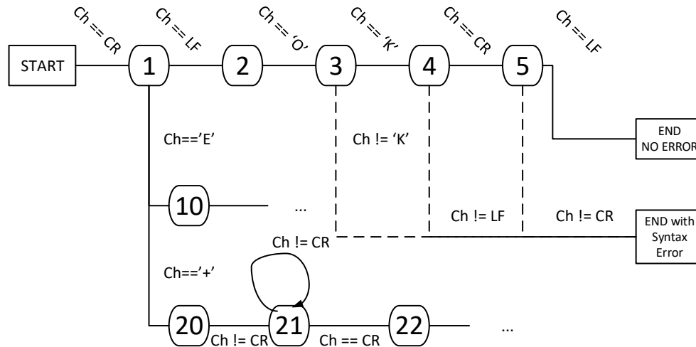
Fig. 1-13 Finite state machine for AT command response language
