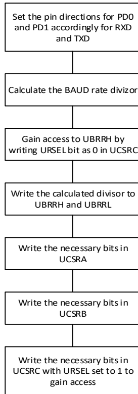
Fig. 4-40 UART initialization flowchart
