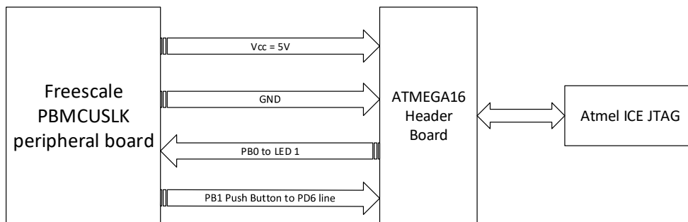
Fig. 4-20 Push button connection block schematic
