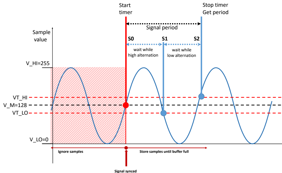
Fig. 2-46 Frequency measurement on positive edge triggering
