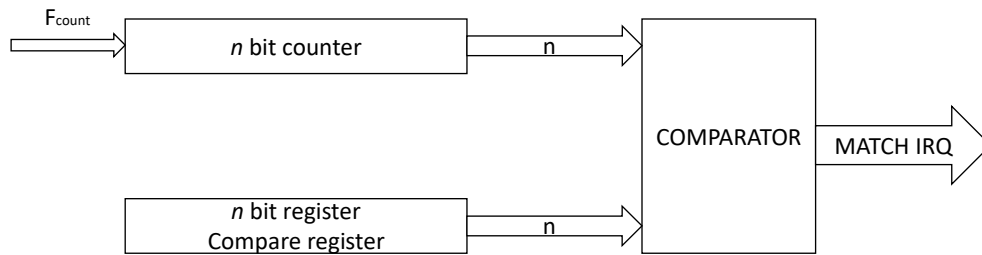
Fig. 4-23 Timer with compare match block schematic
