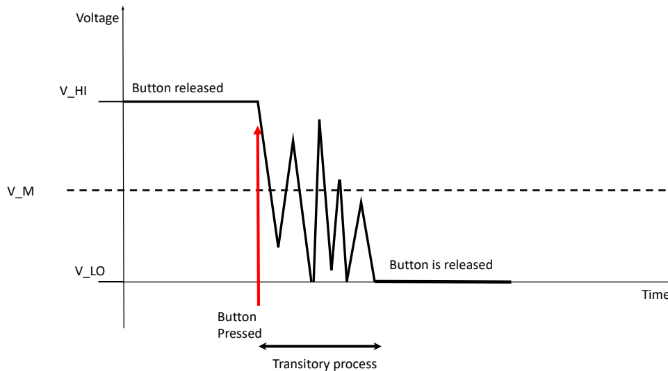
Fig. 4-21 Push-button electrical transient process
