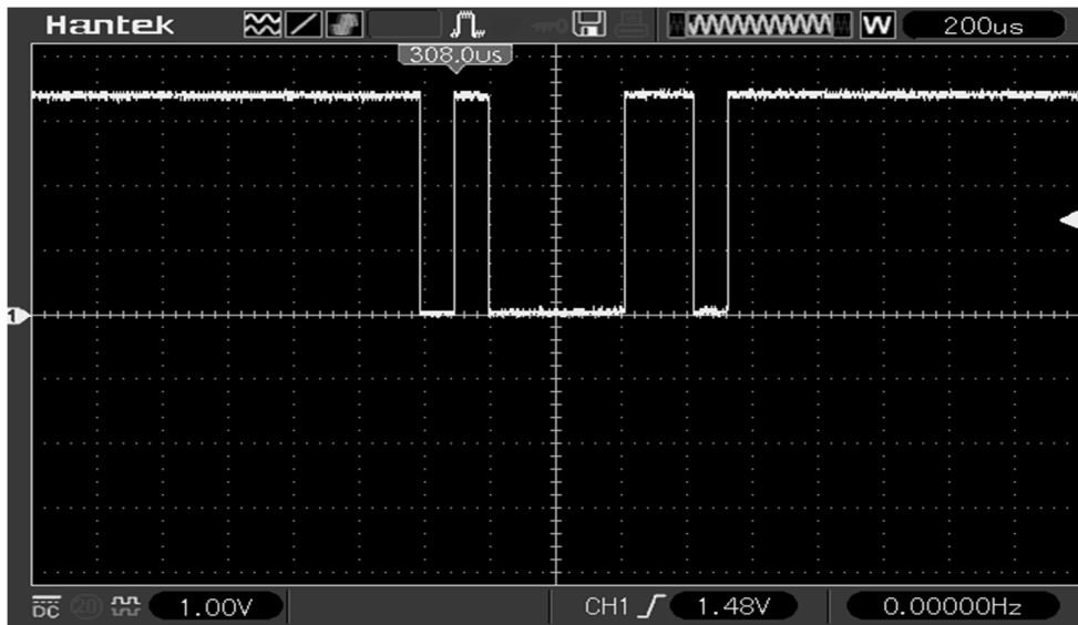
Fig. 2-20 UART character serialization
