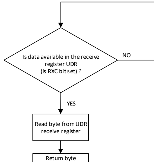
Fig. 4-46 UART receive flowchart
