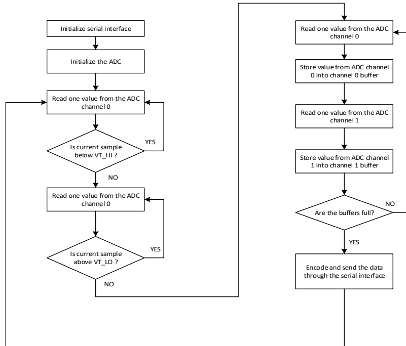
Fig. 2-42 A 2 channel oscilloscope program flowchart with negative edge trigger using instability interval
