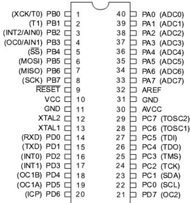
Fig. 4-1 Pinout of ATMEGA16
