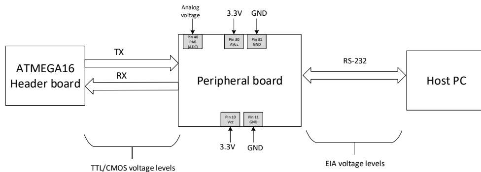
Fig. 2-29 ADC connection block diagram
