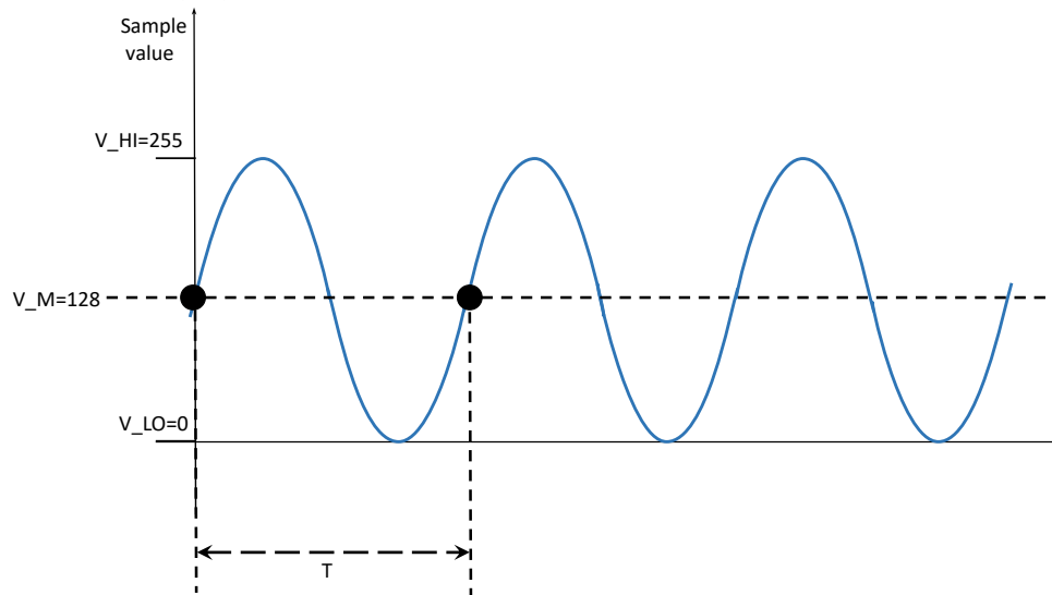
Fig. 2-44 Period definition
