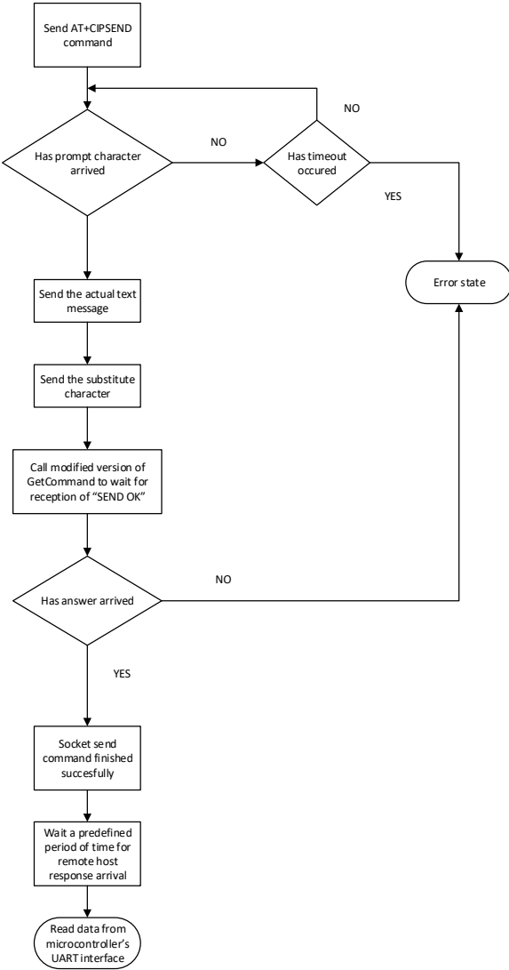
Fig. 1-23 Socket transaction state chart
