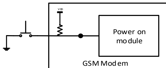
Fig. 1-7 GSM modem power on logic
