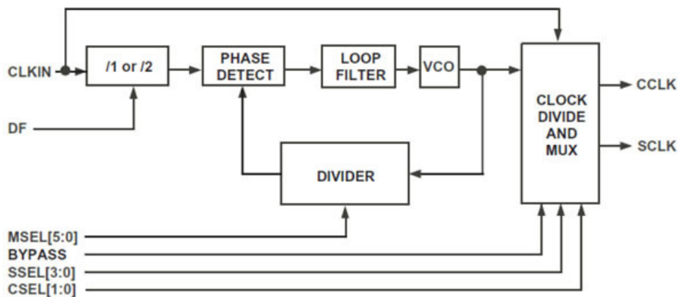
Fig. 3-4 GPIO Blackfin BF537 clock generation diagram [20]
