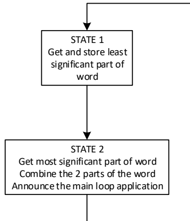
Fig. 2-51 UART 16 bit word reception finite state machine
