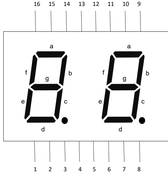
Fig. 4-30 Kingbright DA04-11EWA two digit 7 segment display module pinout
