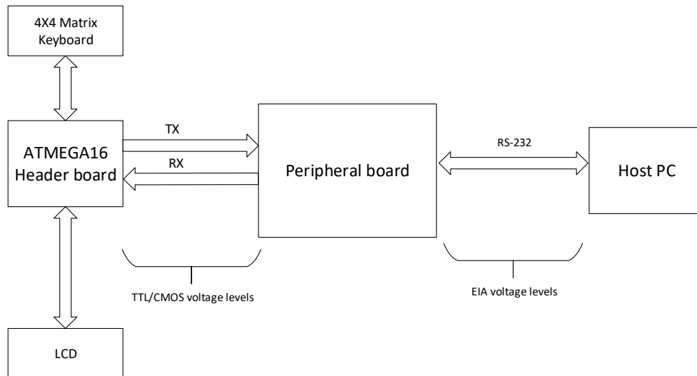
Fig. 4-51 Block schematic
