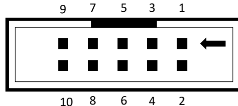
Fig. 1-5 2x5 pin connector orientation and pin numbering
