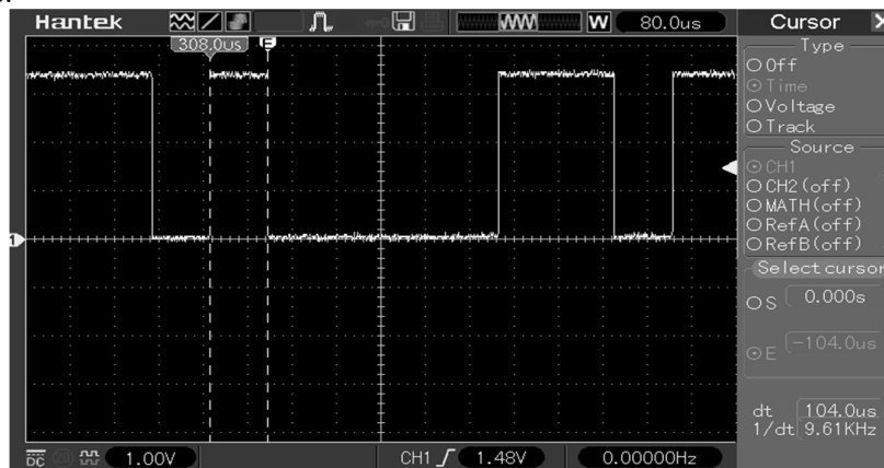
Fig. 4-38 UART bit measurement
