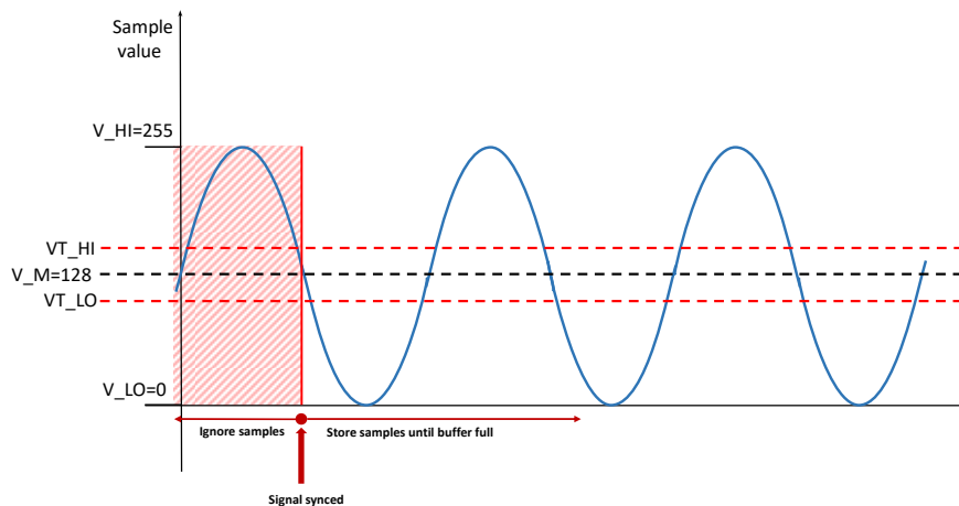
Fig. 2-40 Negative edge trigger using instability interval
