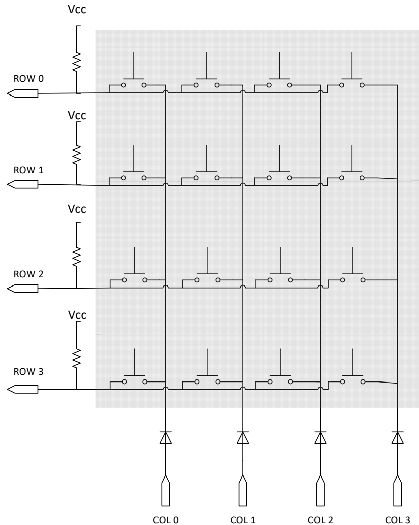
Fig. 4-33 4x4 Matrix Keyboard Schematic
