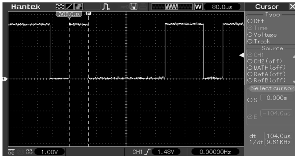
Fig. 2-21 UART bit measurement
