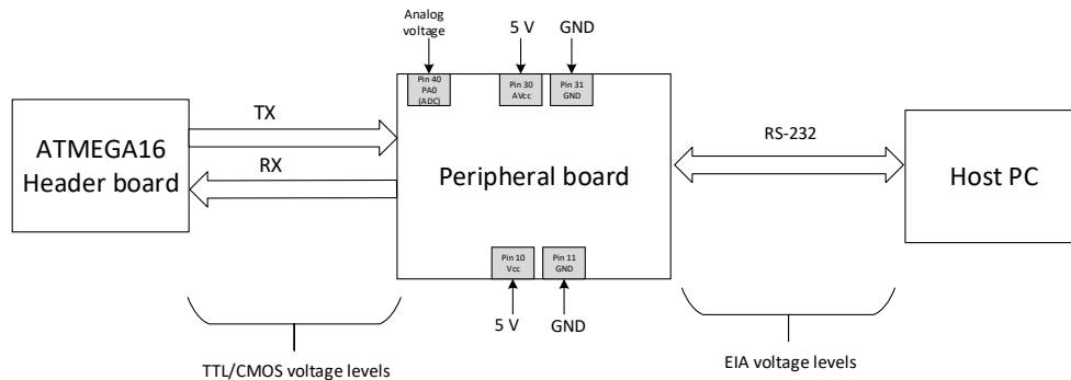
Fig. 4-52 ADC connection block diagram
