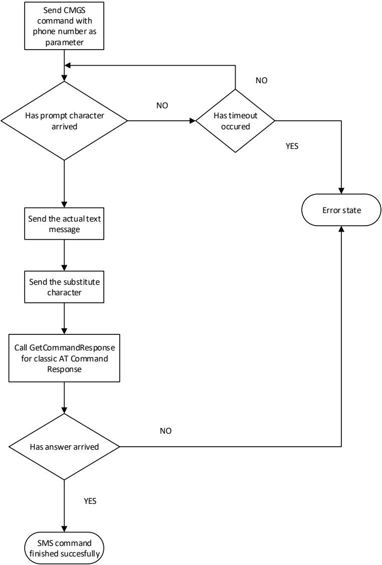
Fig. 1-21 SMS Send state chart
