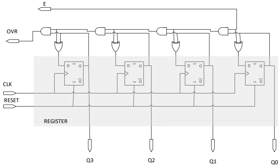
Fig. 4-22 Counter block schematic
