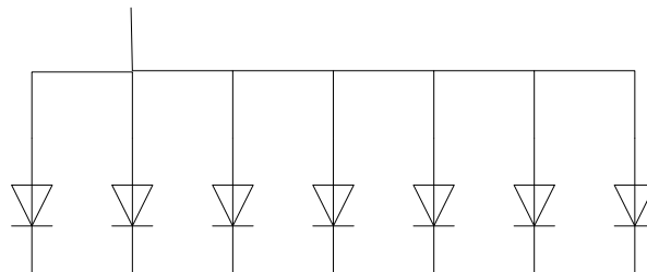
Fig. 4-27 Common anode segment connection
