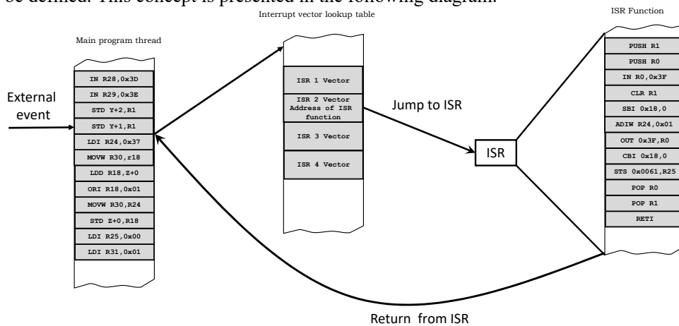
Fig. 4-25 Vectored interrupt diagram
