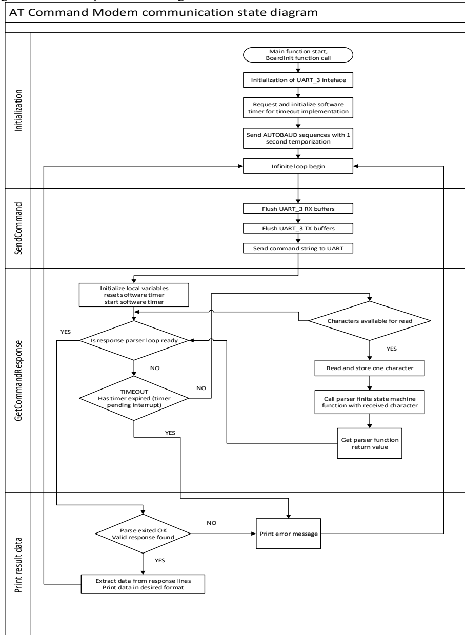
Fig. 1-20 GSM Modem AT command language communication software diagram
