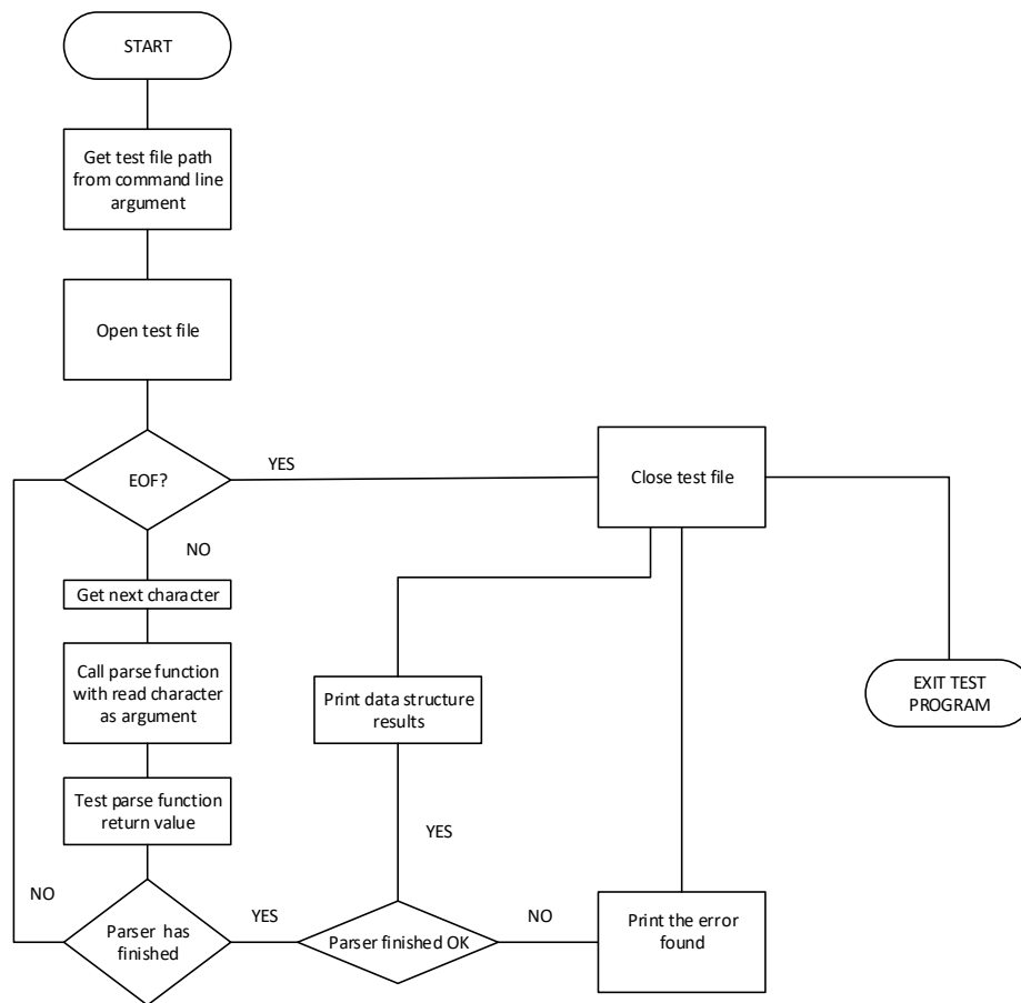
Fig. 1-15 AT command parser test program state diagram
