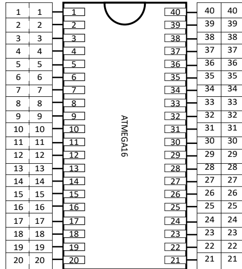
Fig. 2-5 ATMEGA16 header board block schematic
