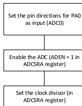
Fig. 2-30 ADC initialization flowchart
