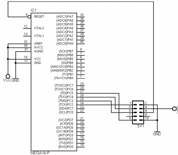
Fig. 2-3 ATMEGA16 JTAG connection
