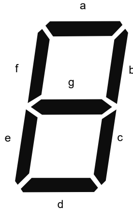
Fig. 4-28 Digit segment notation
