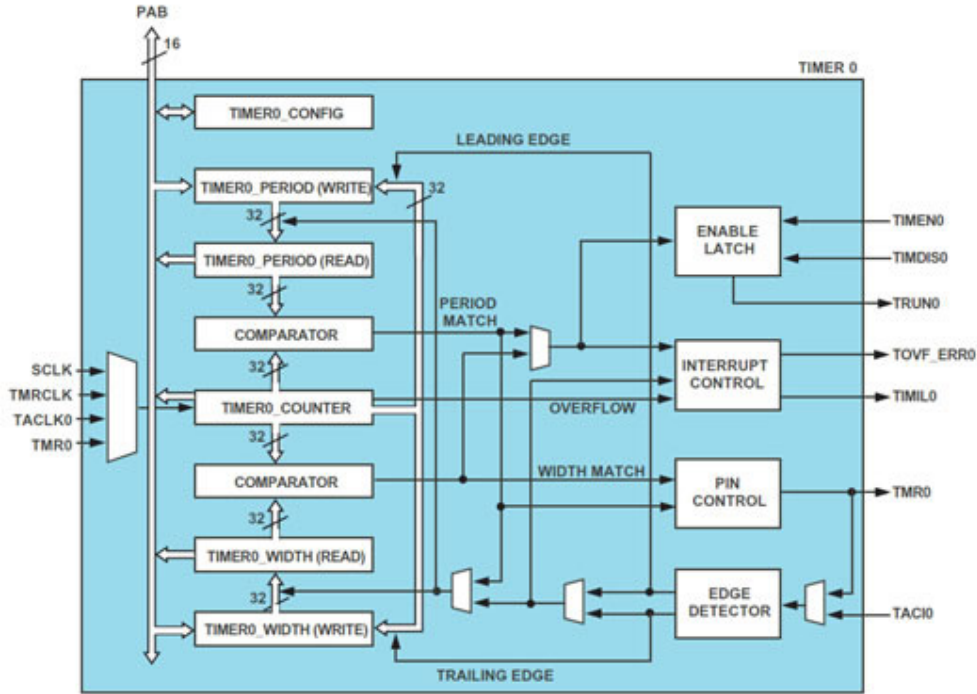
Fig. 3-6 Blackfin BF537 timer internal structure [20]
