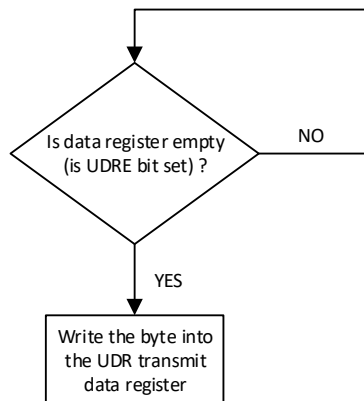
Fig. 4-41 UART transmit flowchart
