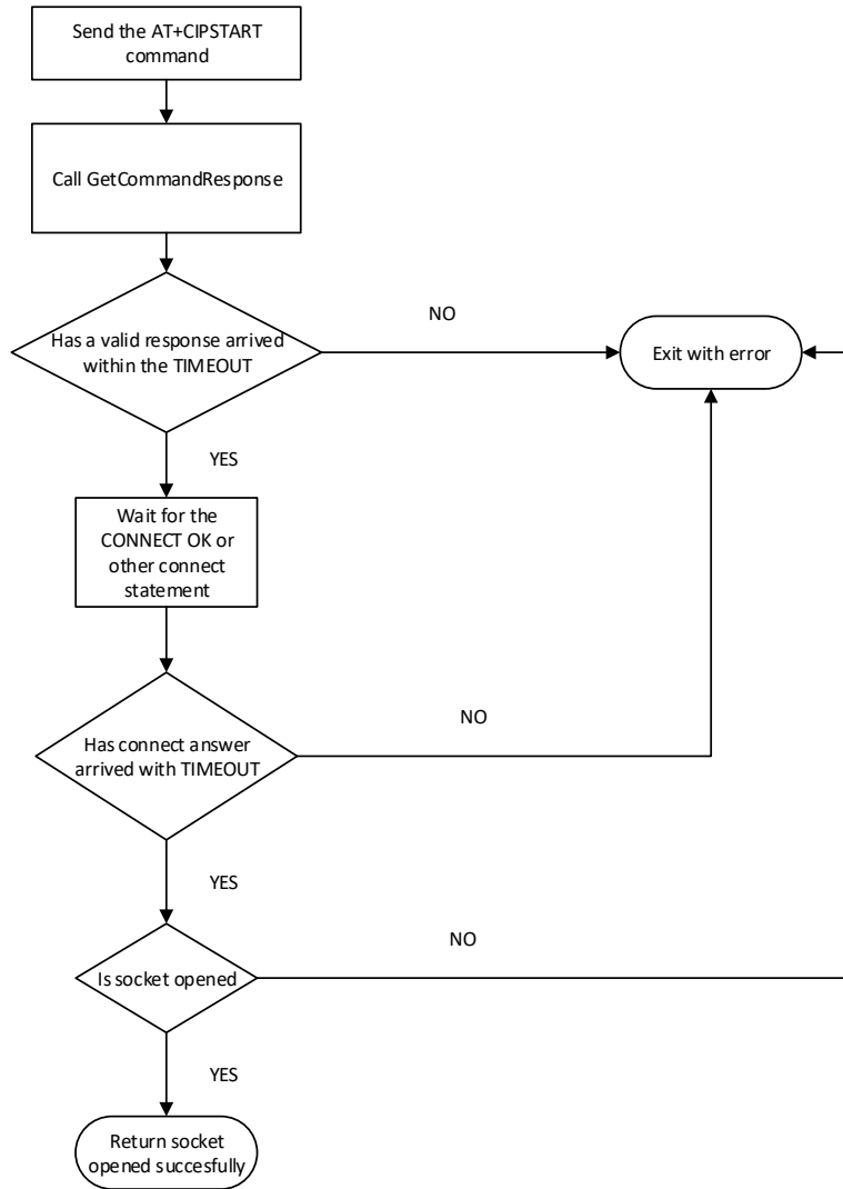
Fig. 1-22 Socket opening state diagram
