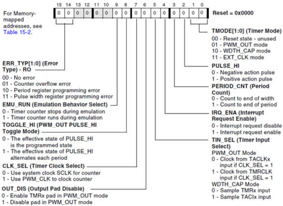
Fig. 3-9 Blackfin BF537 timer configuration register structure [20]
