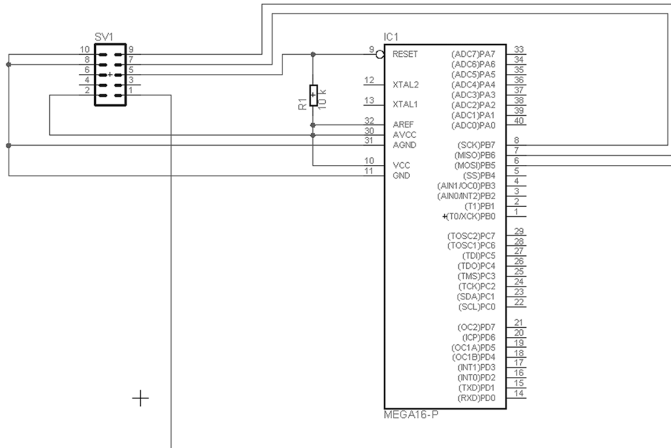
Fig. 4-2 ATMEGA16 ISP connection
